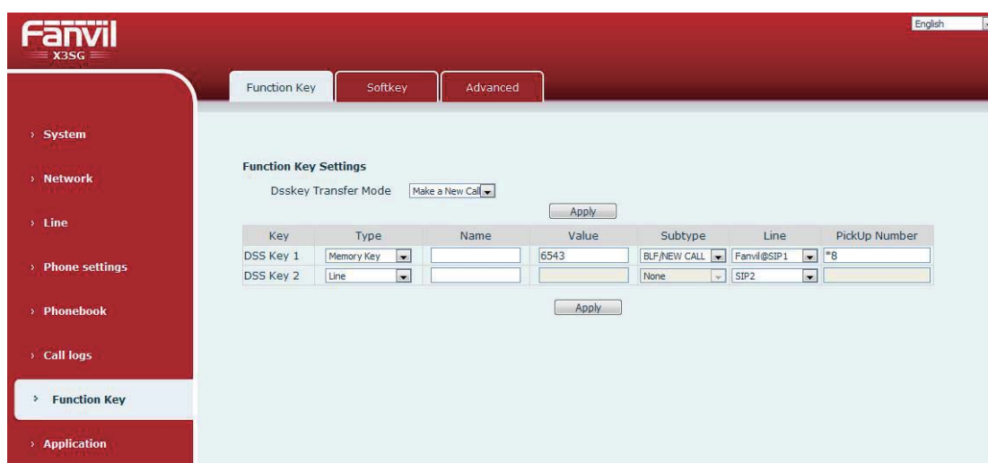
Picture 61 - Web page configuration BLF function key
