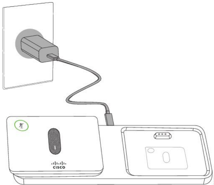
Figure 7: Wireless Microphone Charging Cradle Installation
