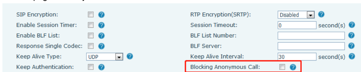
Picture 56 - Page Settings blocking anonymous call
