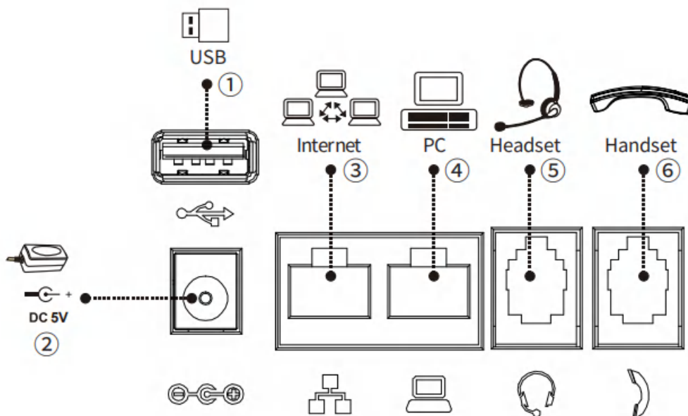
Picture 3 - Connecting to the Device
